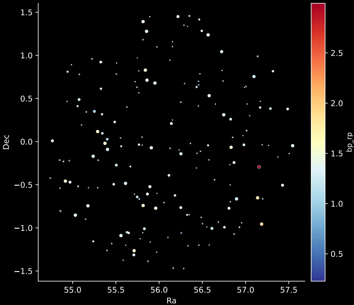
APOGEE DR17 Field: [050-29_MGA] Stars: 176
