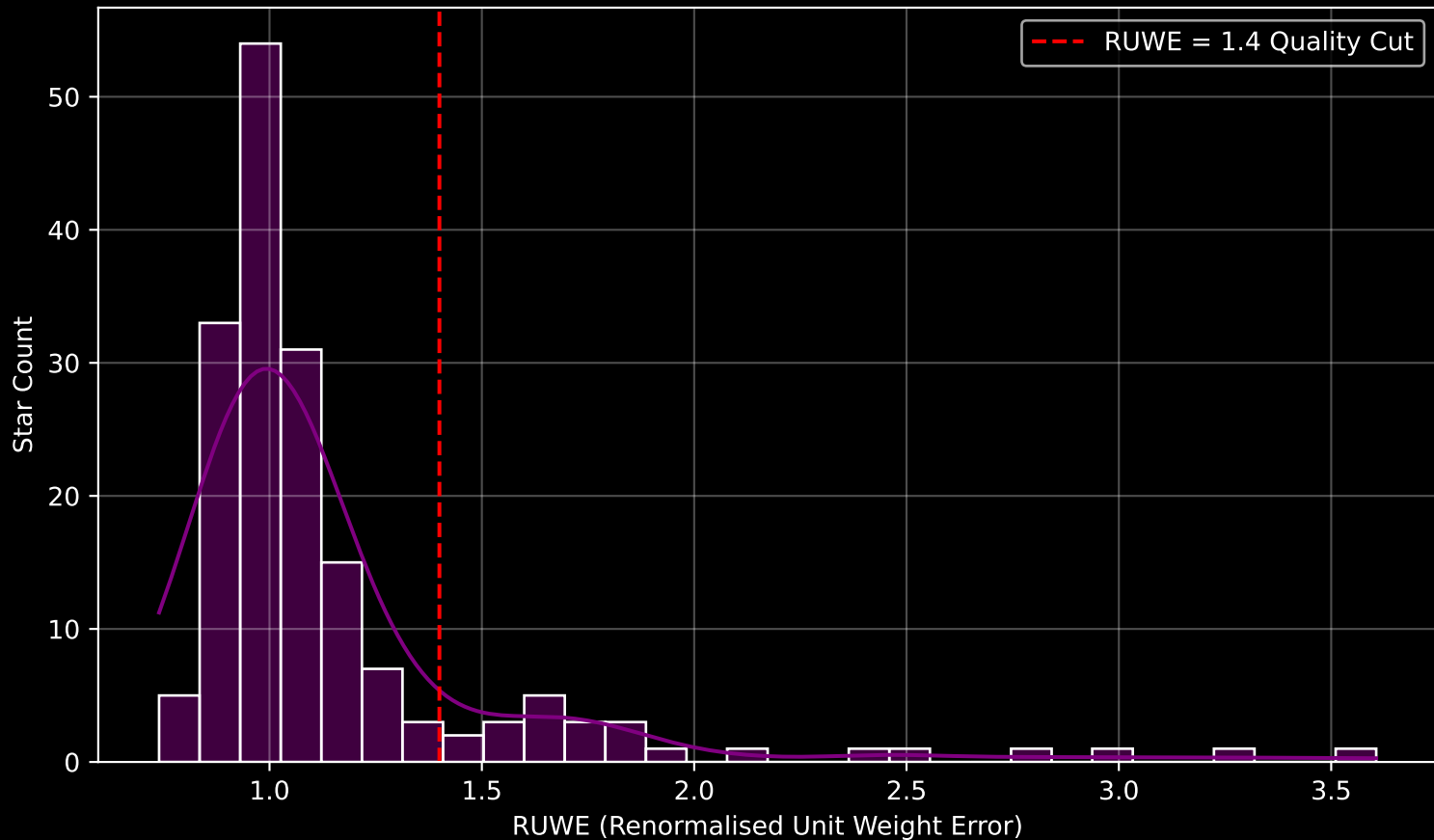
GAPOGEE DR17 Field [050-29_MGA] RUWE Distribution (n= 172)
