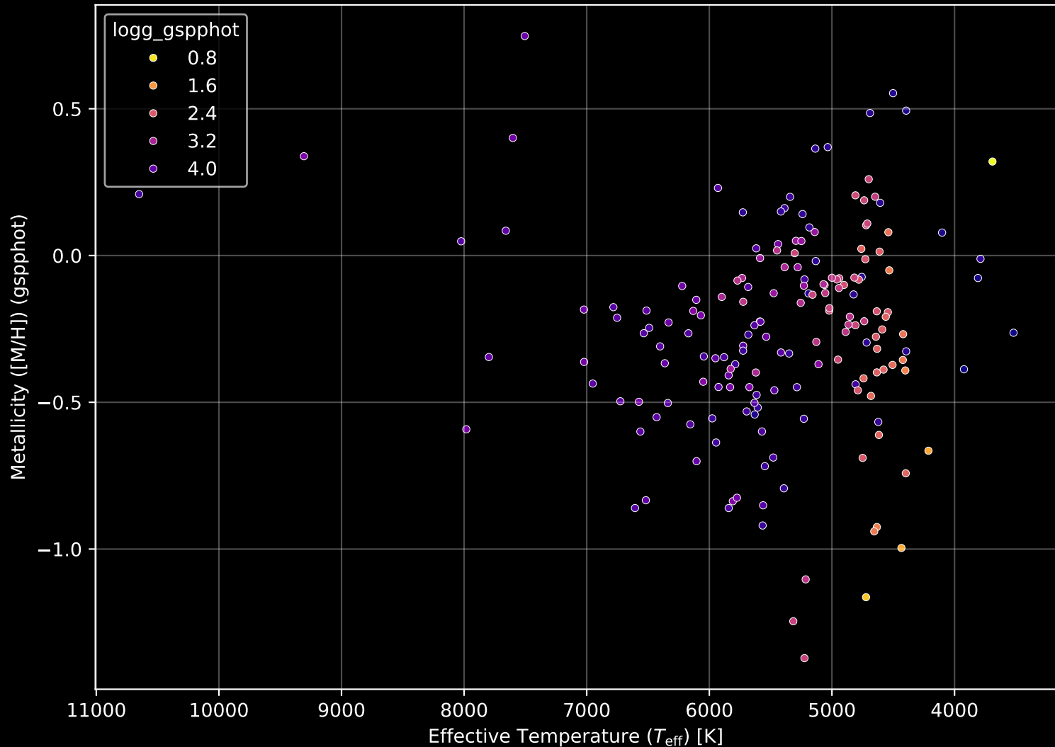
APOGEE DR17 Field: [050-29_MGA] Stellar Population Parameters (n= 176)
