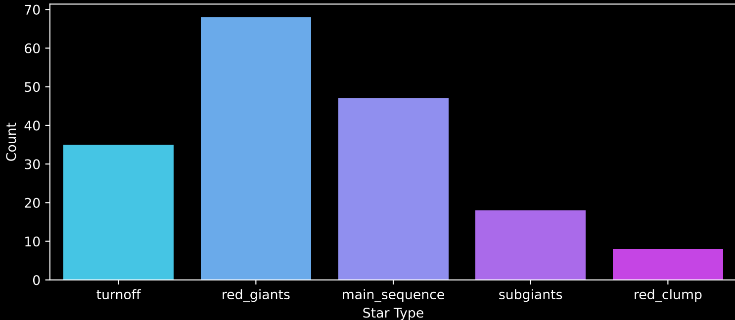
APOGEE DR17 Field: [050-29_MGA] Count plot of Star Type
