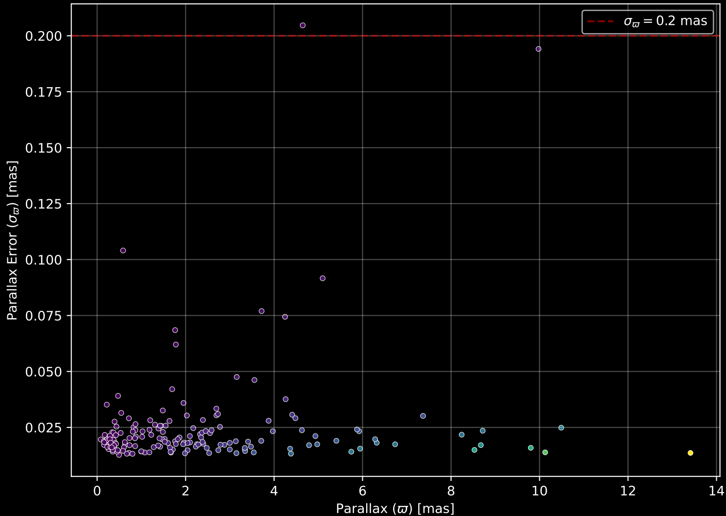
APOGEE DR17 Field: [050-29_MGA] Parallax Quality (n= 176)
