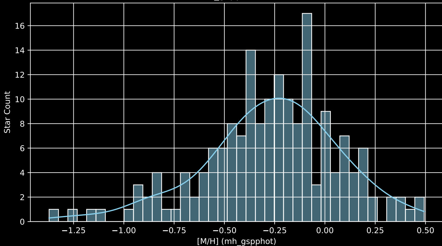
APOGEE DR17 Field: [050-29_MGA [M/H] (mh_gspphot) (n= 174)
