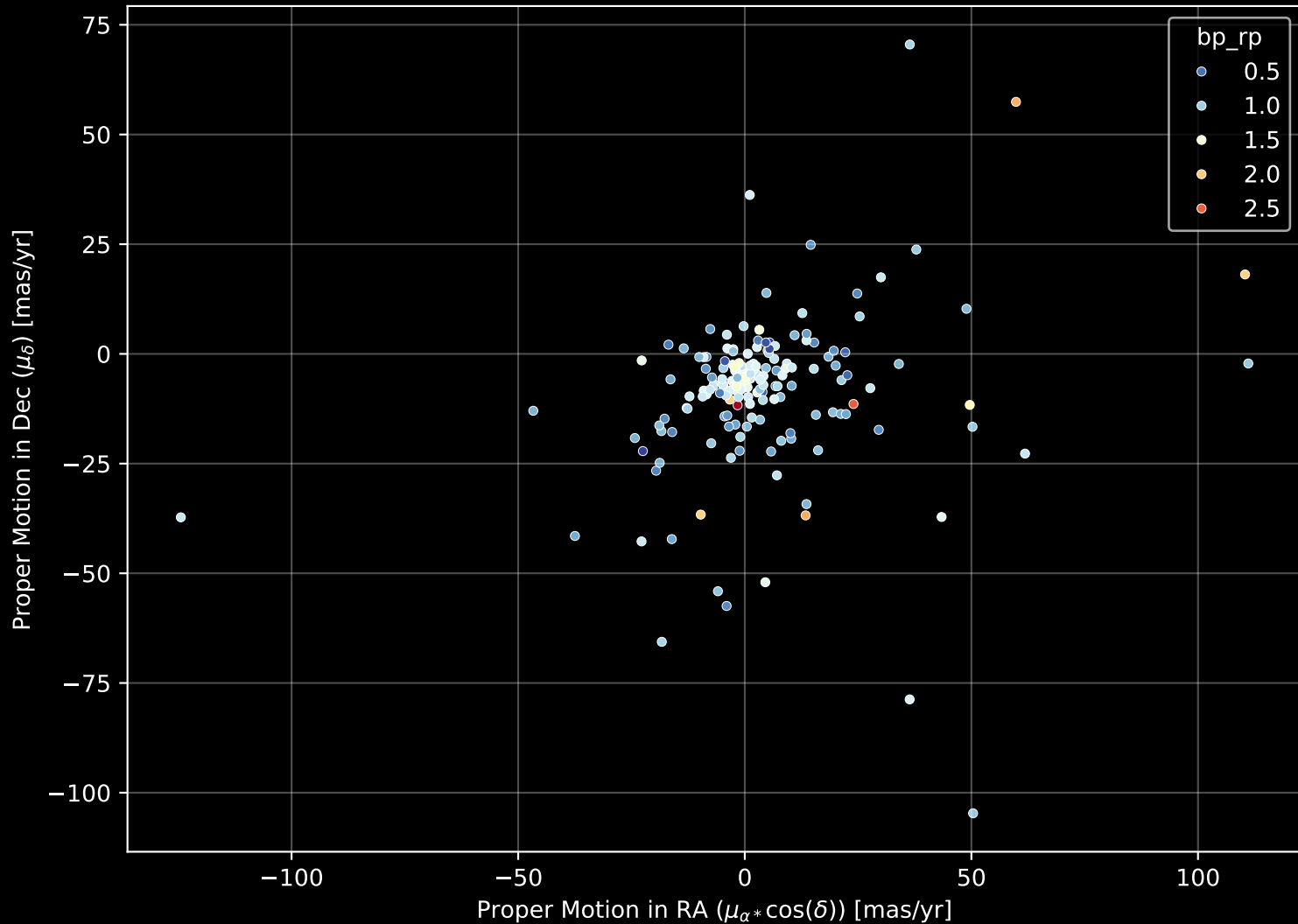
APOGEE DR17 Field: [050-29_MGA] Proper Motion Diagram (n= 176)
